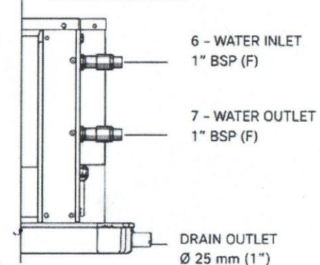
CONNECTION DETAIL
