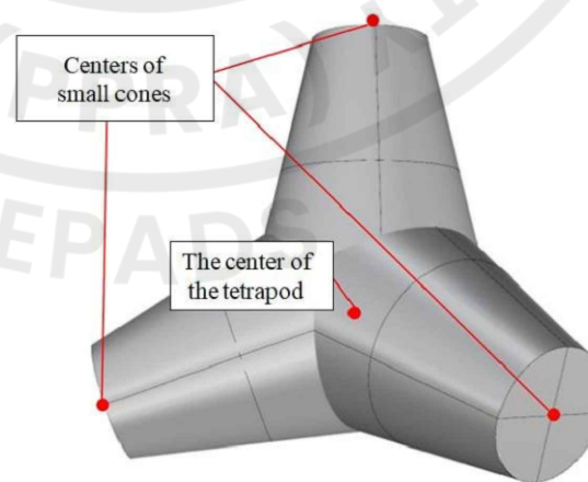
TETRAPOD 3D VIEW
