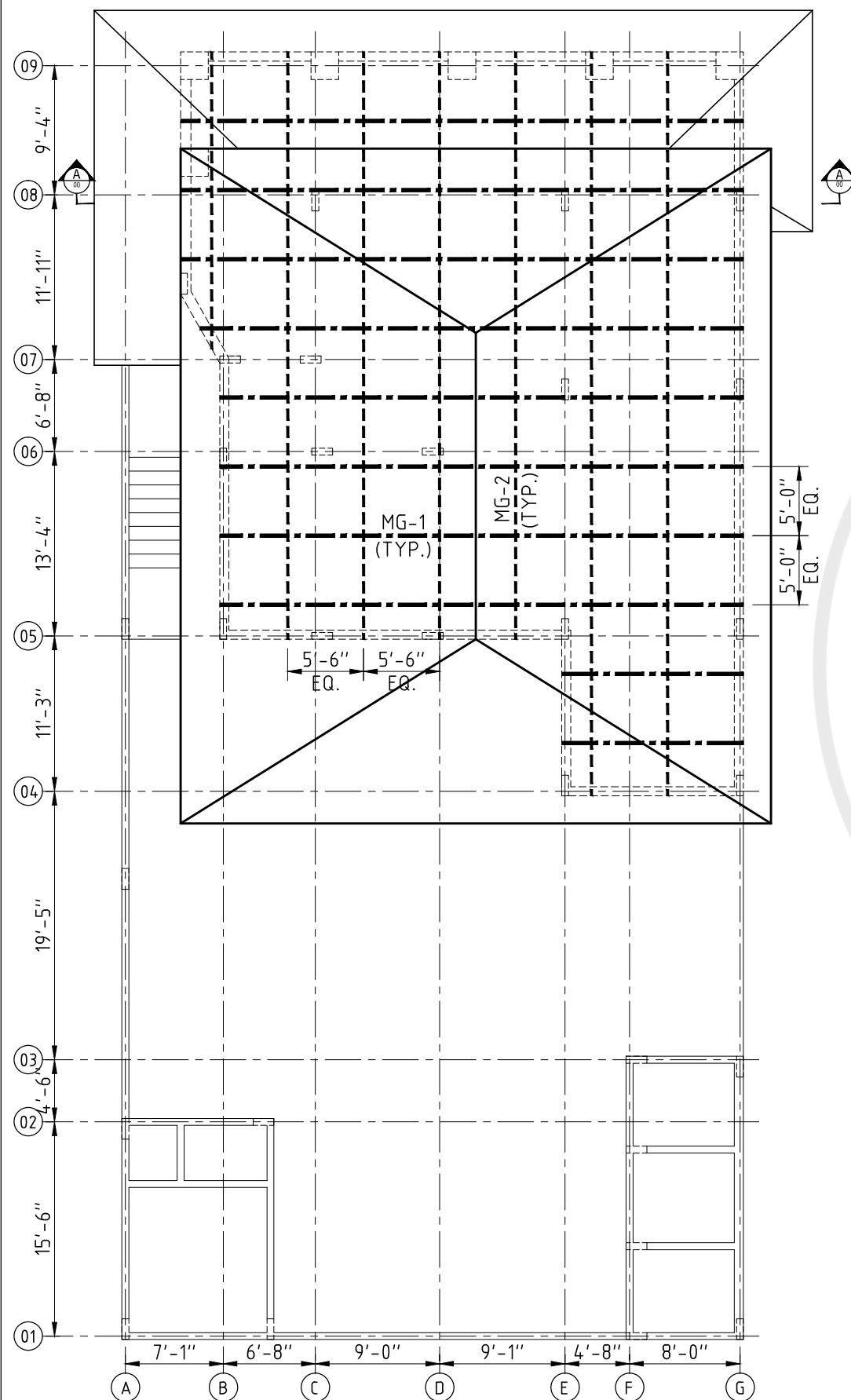
ROOF MS GIRDER LAYOUT PLAN SCALE: 3/32"=1'-0"
