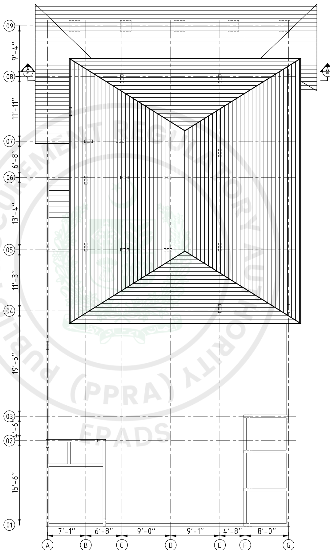
ROOF SLAB LAYOUT PLAN SCALE: 3/32"=1'-0"
