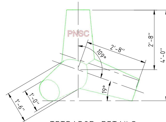
TETRAPOD DETAILS SCALE: 1/64"=1'-0"
