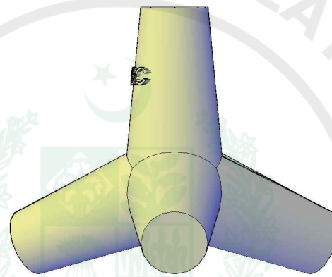
RIGHT VIEW OF TETRAPOD SCALE: 1/64"=1'-0"
