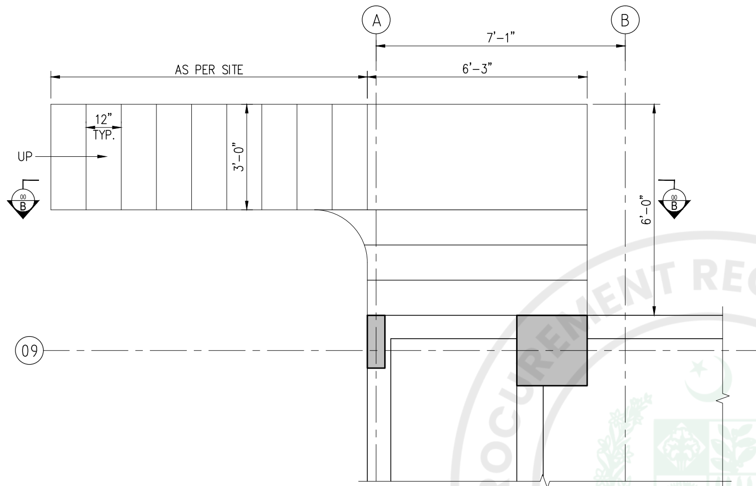
STAIR CASE LAYOUT PLAN SCALE: 3/8"=1'-0"
